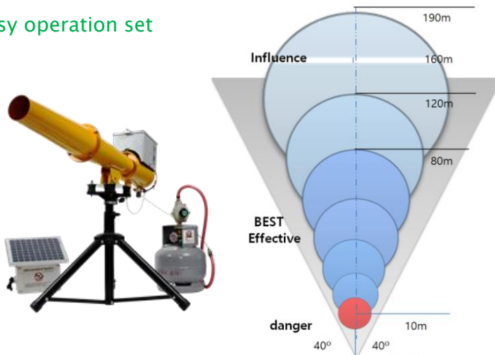
LPG Cannon 1803A Bird repelling effect by distance
